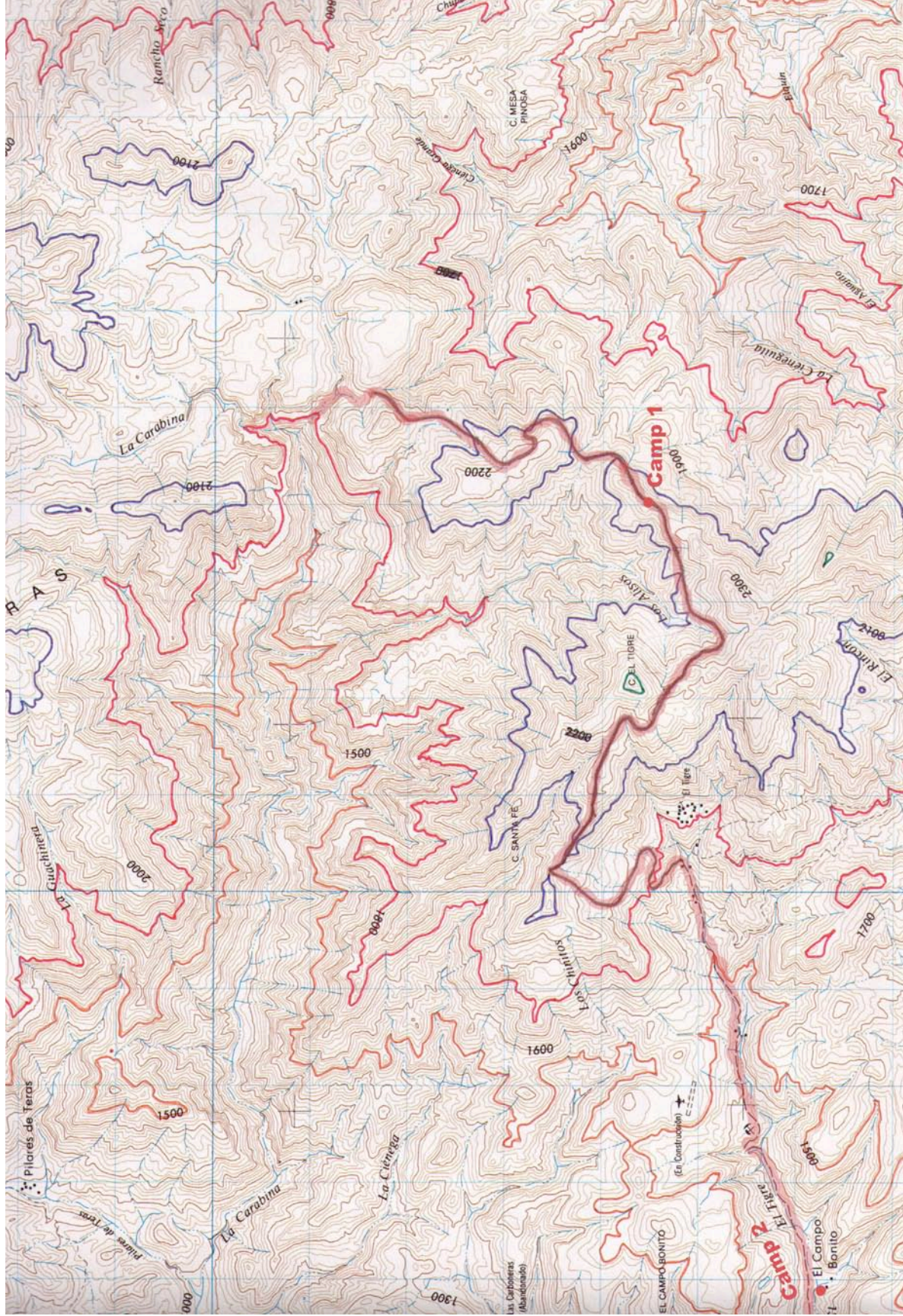
Map 2. Corridor of travel in the Sierra El Tigre
